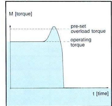
Switching behaviour
