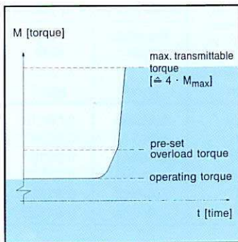
Switching behaviour
