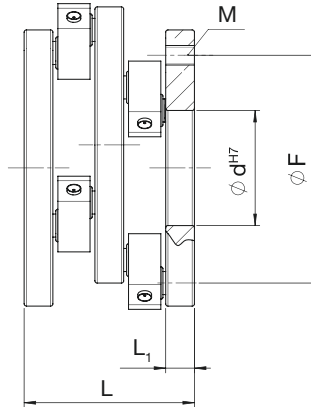
55: Flange mounting
