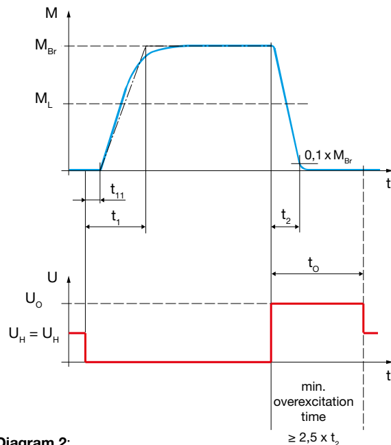
Diagram 2: Switching times Type 899. _ _ _ . _2, brake operation with overexcitation voltage
