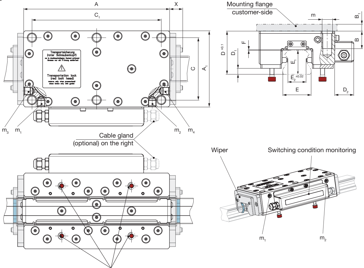
Fig. 1 Transportation lock
