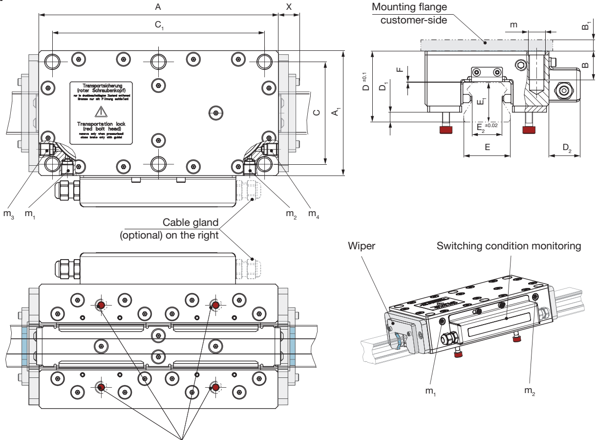
Fig. 3 Transportation lock
